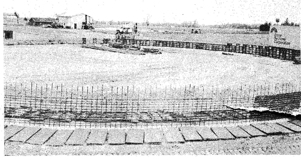
GOING UP: Additional storage space is under construction at the Elkton Plant of Co-operative Elevator. The round shape will provide the foundation to new dome style storage buildings. Huge vinyl "balloons" are inflated and covered with polyurethane insulation and steel to give the domes their unique shape. Elevator officials hope construction will be complete in mid-July.
