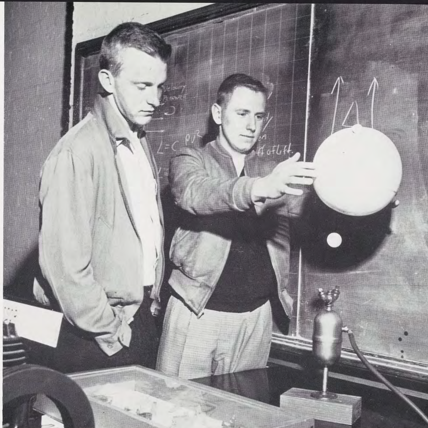
The air flow principle is demonstrated by holding a ping pong ball in mid air.
