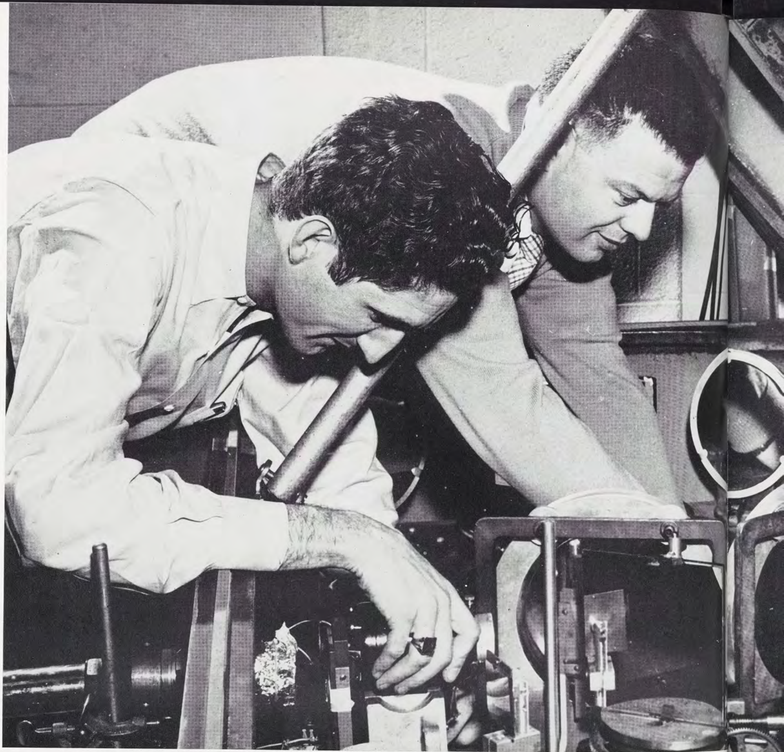
Physics student Carleton Savage and Professor Edwards make adjustments on an infrared spectrograph. All components in this machine are enclosed in a high vacuum tank when in use.
