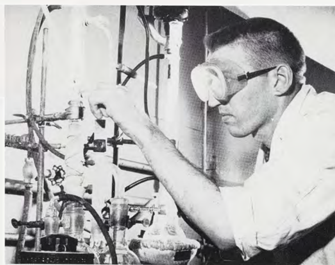
A fractionation process occupies the attention of chemistry graduate student John Regan. He is causing certain components of the compound to evaporate by raising the temperature.
