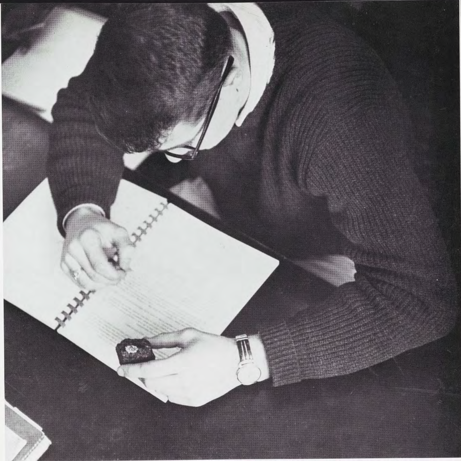
A natural science student pores over his text book, trying to identify a sample rock for his laboratory report.
