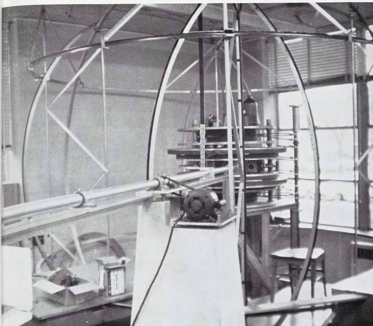
This Beta-ray spectrometer, located in the Physics-Mathematics Building, is used to study radioactive nuclei and the low energy properties of nuclear transitions.
