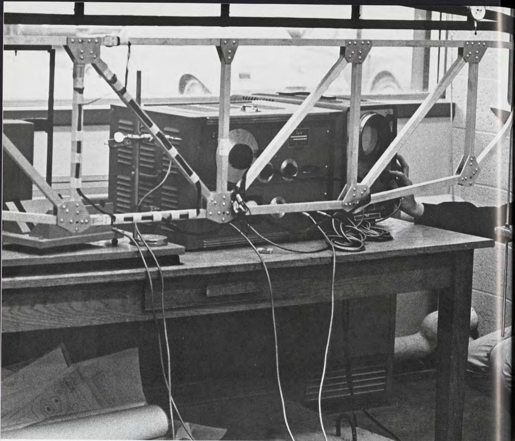
An intricate model of a bridge enables this student to test the points of stress and strain.
