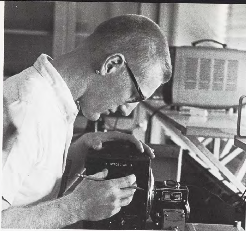
A lab student uses a stroboscopic light to measure the speed of an electric motor's rotation.
