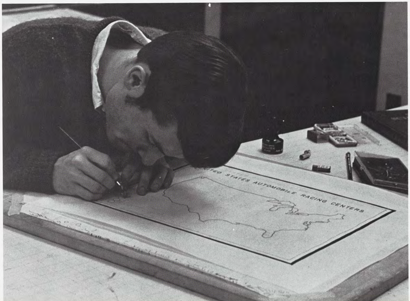
The elements of map construction allow the geographer to understand the earth's physical and cultural phenomena.
